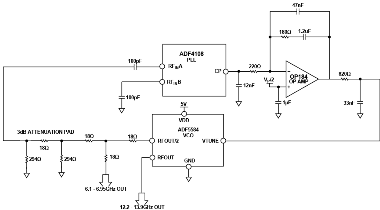
Figure 22. ADF5584 used with ADF4108 in a Microwave 13.0 GHz PLL Loop
