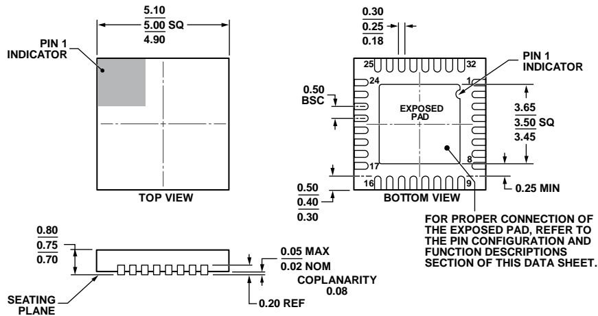
COMPLIANT TO JEDEC STANDARDS MO-220-WHHD. Figure 23. 32-Lead Lead Frame Chip Scale Package [LF CSP_WQ] 5 mm x 5 mm Body, Very Thin Quad (CP-32-13) Dimensions shown in millimeters
